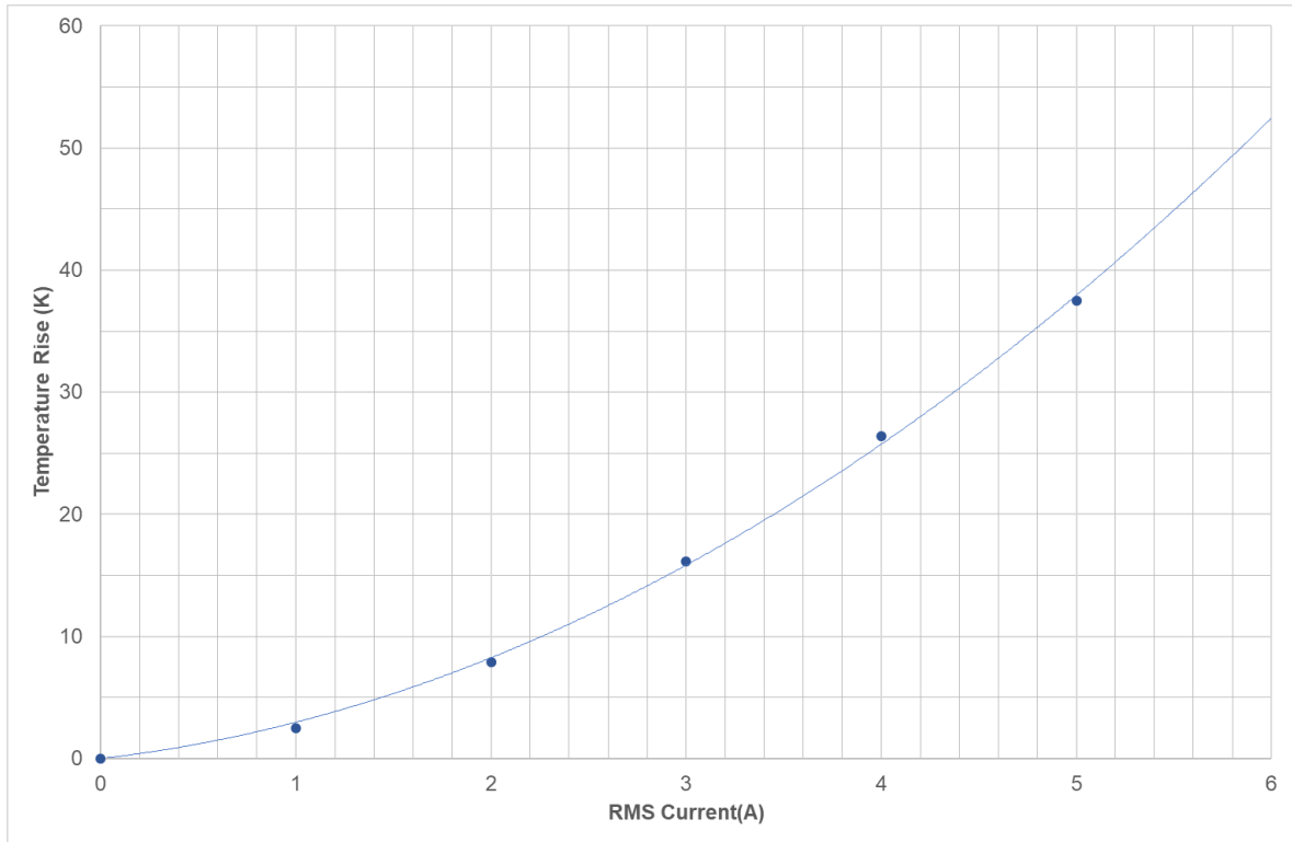
Fig 12: Temperature rise in DMF4B5R5G105M3DTA0 with RMS current
